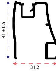
Agron - Amata Yan Panel Ayar Profili
