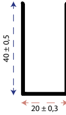
Agron - Amata Yan Panel Duvar Profili
